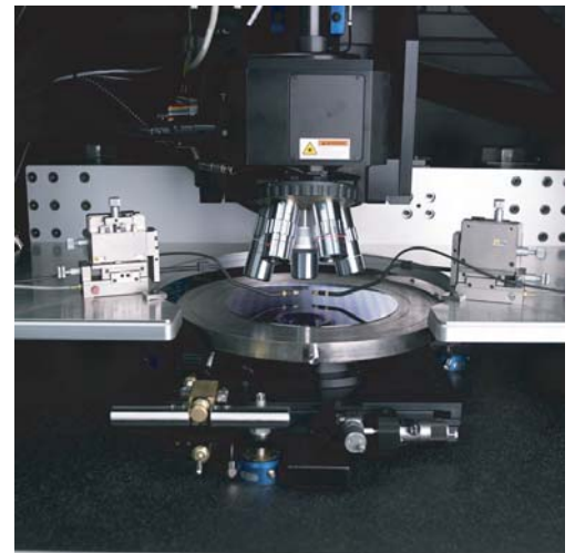
Laser Scanner and Microscope Module
